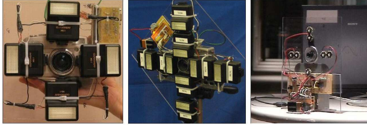
Figure 1: Multi-flash camera setups used in [13] for depth edge detection. From left to right: 4-flash setup, 8-flash setup and dynamic scenes setup. Our goal in this paper is to exploit multi-flash imaging for specular reflection reduction.
